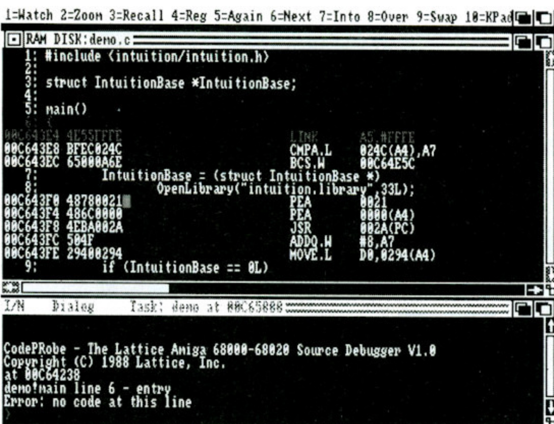
■ Lattice C at work. The compiler is, of course, an essential part of the use of a programming language, so choose a compiler carefully.
